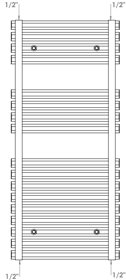
Back View
