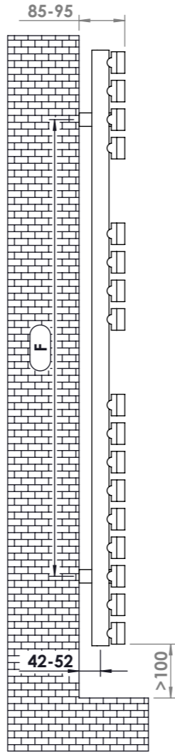
Side View
